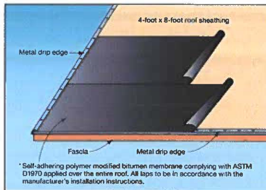
Sealed Roof Deck Option #1
